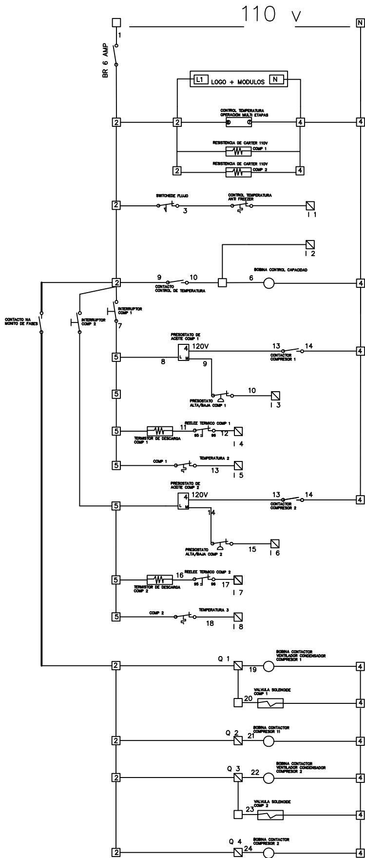
PLANO ELECTRICO DE CONTROL CHILLER SALON SAPAN Sebastian Ocañana Hidalgo Frey Ramirez Rodriguez
